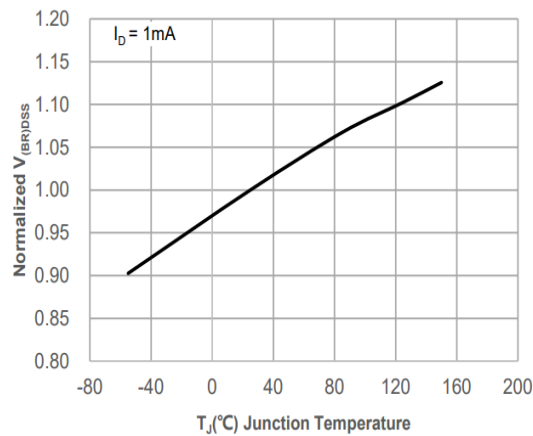
Figure 5: Normalized Breakdown voltage vs. Junction Temperature
